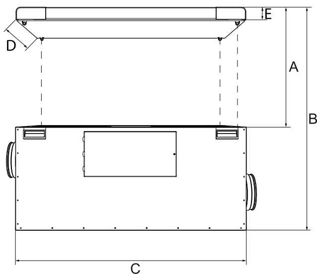
Monteringsavstand for HERU S
