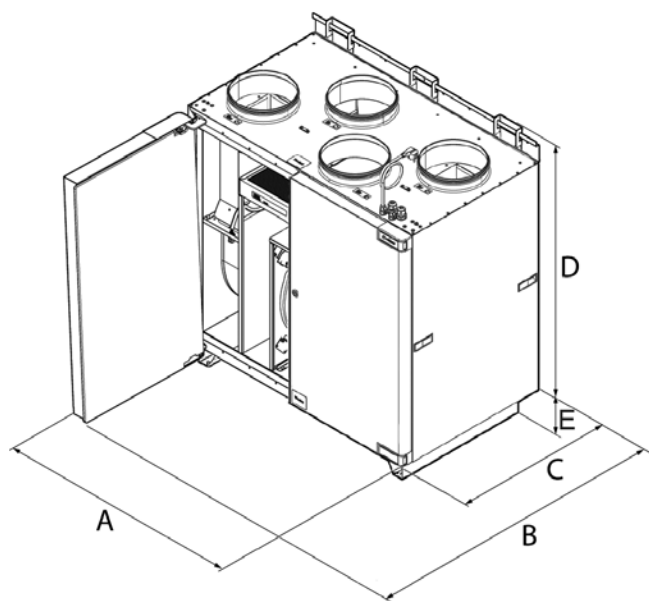
Mounting distance for HERU T
