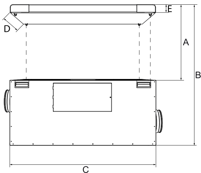
Mounting distance for HERU S
