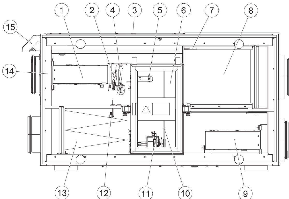
Fig. 9 Internal components
