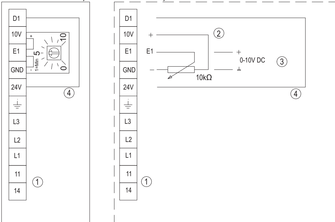
Internal potentiometer
