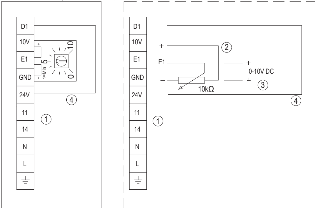
Internal potentiometer
