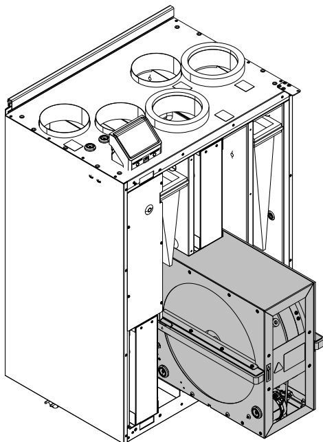
Fig. 4 Heat exchanger
