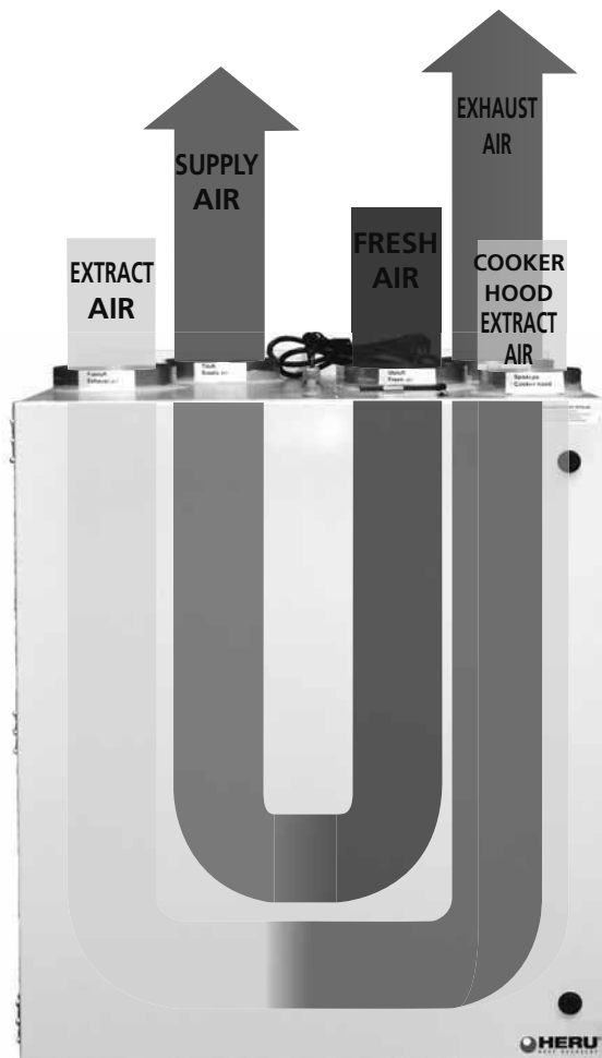
LEFT HANDING APPLICATION: HERU®62 T, 90 T, 95 T EC, 115 T, 140 T WITH COOKER HOOD CONNECTION.
