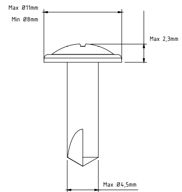
Mounting screw
